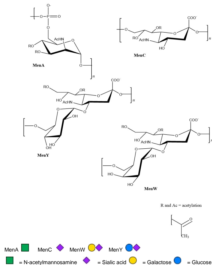
Figure 1. Chemical structures of monosaccharide units of meningococcal polysaccharides for which there are currently glycoconjugate vaccines. Sites of potential O-acetylation is indicated by R groups. The monosaccharide symbols follow the Symbol Nomenclature for Glycans (SNFG) according to [49].
