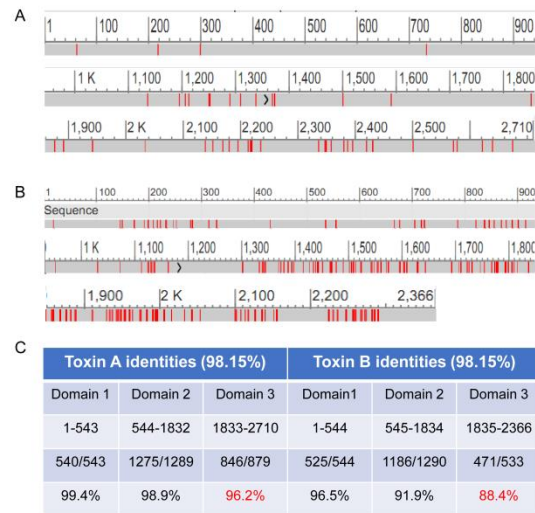
Figure S1. Blast results of toxin amino acids sequence in CD bacterium strain VPI10463 and strain ATCC BAA-1870. (A) Toxin A; (B) Toxin B; (C) The complete toxin A and toxin B. Red parts in A and B are different amino acids. Domain 3 is RBD of toxin.
