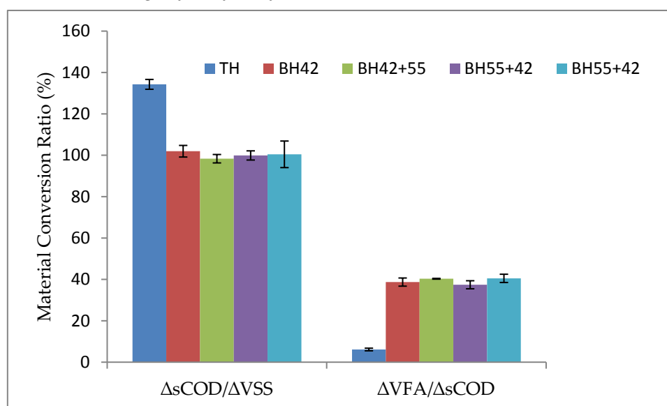
Figure 4. Material conversion ratios of \Delta s\text{COD}/\Delta\text{VSS} and \Delta\text{VFA}/\Delta s\text{COD} due to TH and BH treatments.
