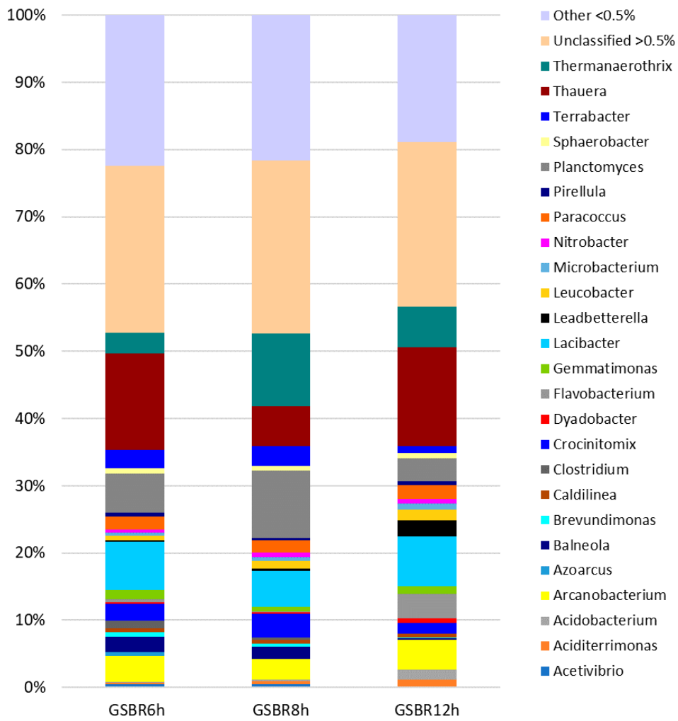
Figure S2. 2SM Bacterial taxa in granular sludge
