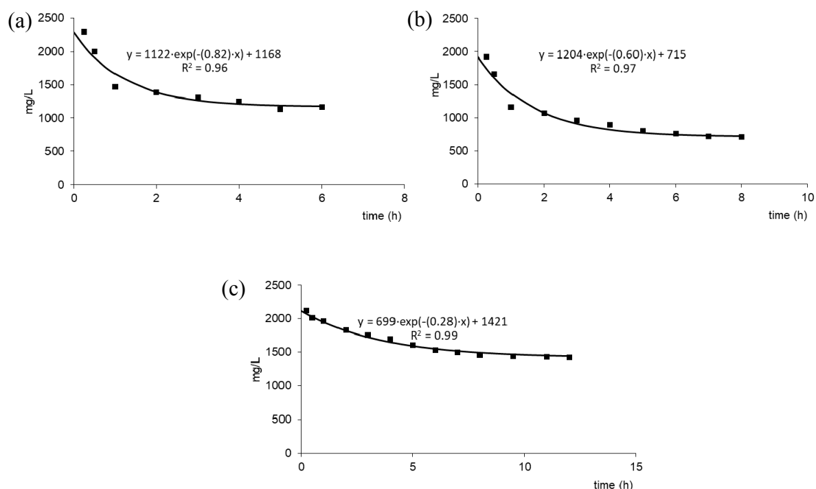
Figure S1. Kinetics of COD removal in the cycle of GSBRe 6h (a), GSBRSrh (b) and GSBRe 12h (c)
