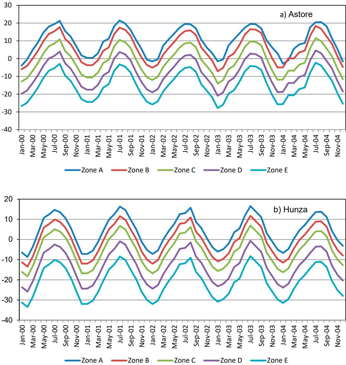
Figure S1. Mean monthly zonal temperature estimated from the available ground data using a lapse rate value for the a) Astore and b) Hunza basins.
