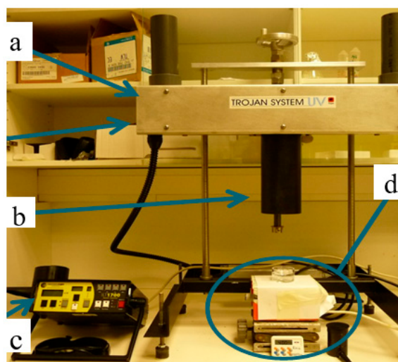
Figure S2. Trojan UV collimated beam system excluding the shutter. a) UV lamp, b) collimated beam, c) Radiometer, and d) water sample with magnetic bar on the stirrer.
