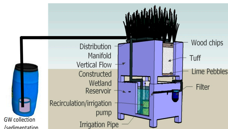
Figure S1. Schematic of the onsite recirculating vertical flow-constructed wetlands (RVFCW) GW treatment system (After Alfiya et al., 2013).
