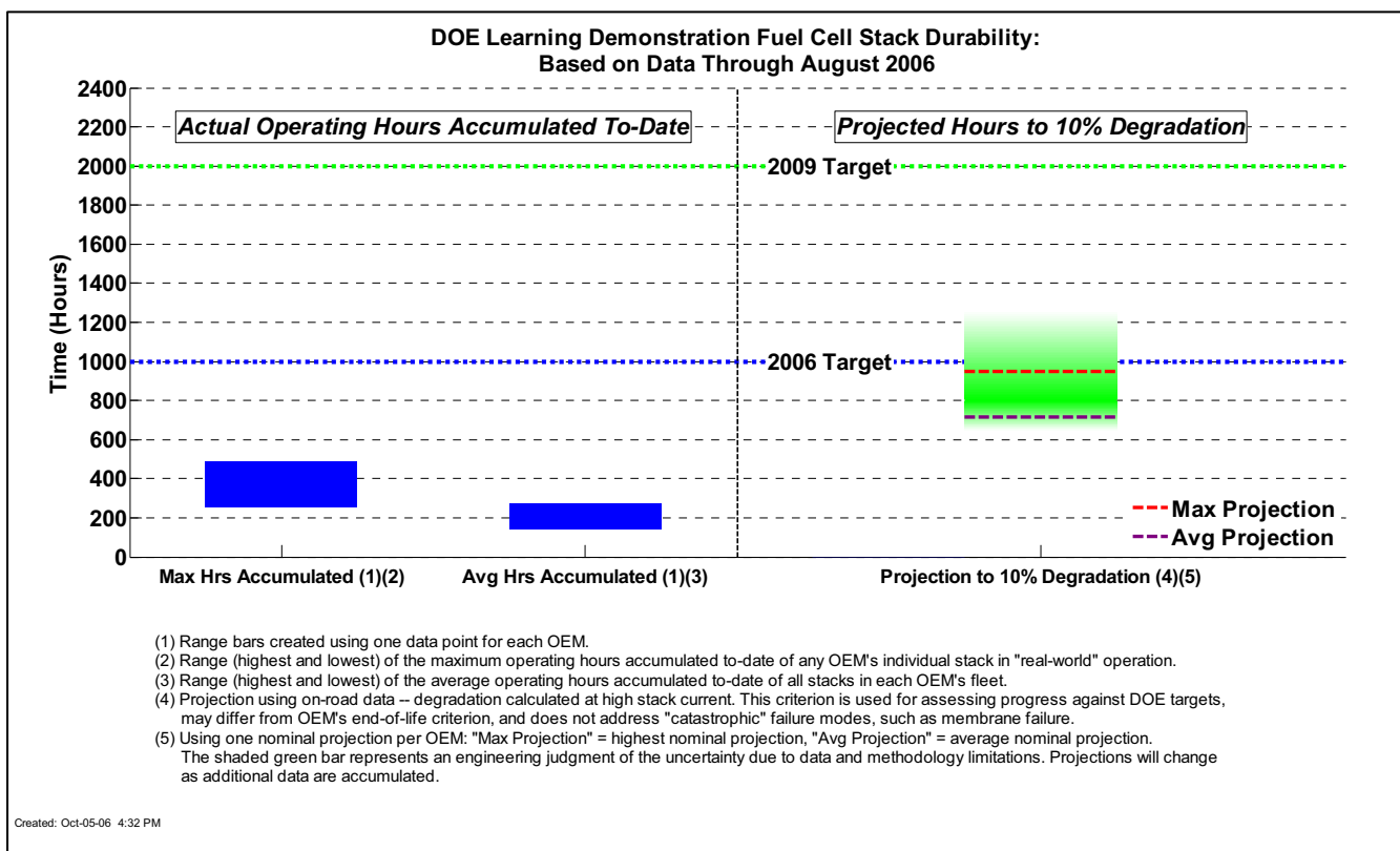
Fig. 7 Accumulated stack operating hours todate and projected time to 10% voltage degradation
