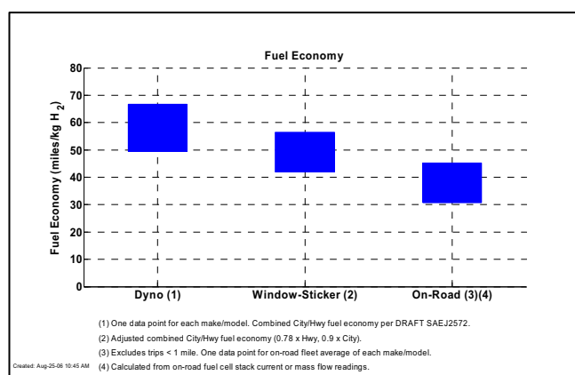
Fig. 5 On-road and dynamometer fuel economy from all four teams
