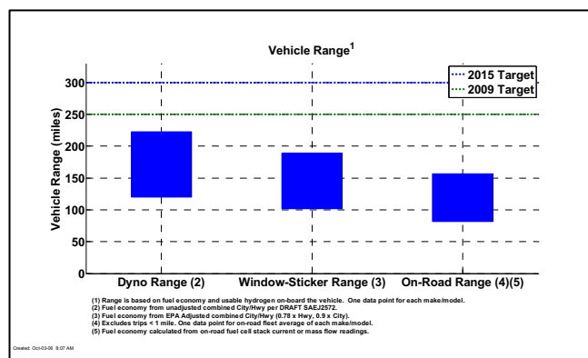
Fig. 6 Vehicle driving range calculated from fuel economy and usable hydrogen
