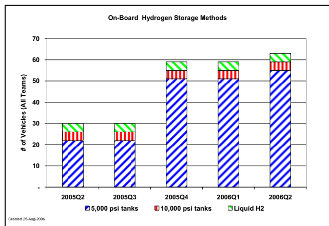
Fig. 8 Number of vehicles by year and quarter using various on-board storage technologies
