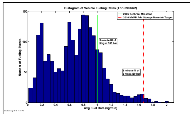
Fig. 10 Vehicle refueling rate histogram
