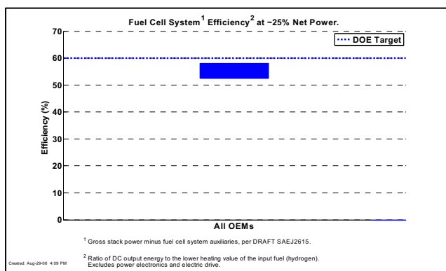
Fig. 4 Range of measured fuel cell system efficiency at 25% net power from all four teams
