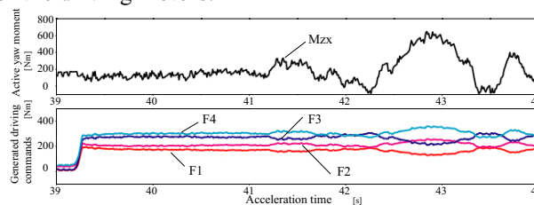
Fig. 10 Time history of the controlled driving torque (according to the generated active yaw moment)
