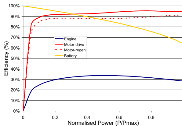
Fig. 5: Efficiency curves used in the PHEV
