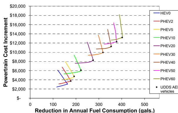
Fig. 9: Incremental costs and annual petroleum consumption for the spectrum of PHEV designs
