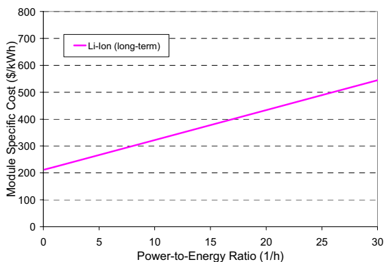
Fig. 7: Battery module cost for Li-Ion technology
