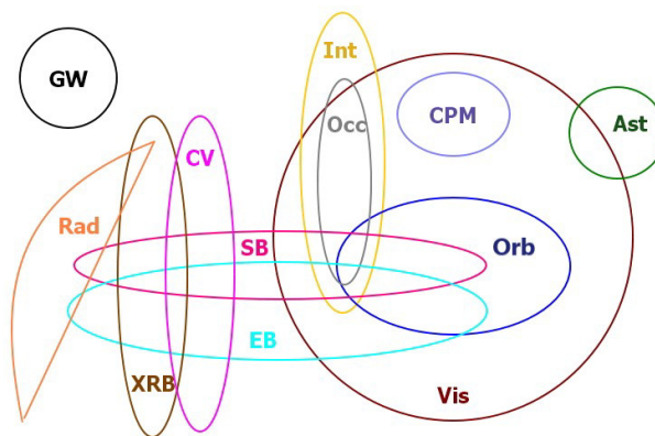
Figure 1. Observational types of binaries. See text for details.
