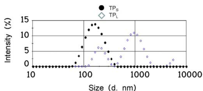
Figure 1. Particle size distribution of intensity measured, by dynamic light scattering analysis. Black circles show the size distribution of \text{TP}_S , and open diamonds of \text{TP}_L .
