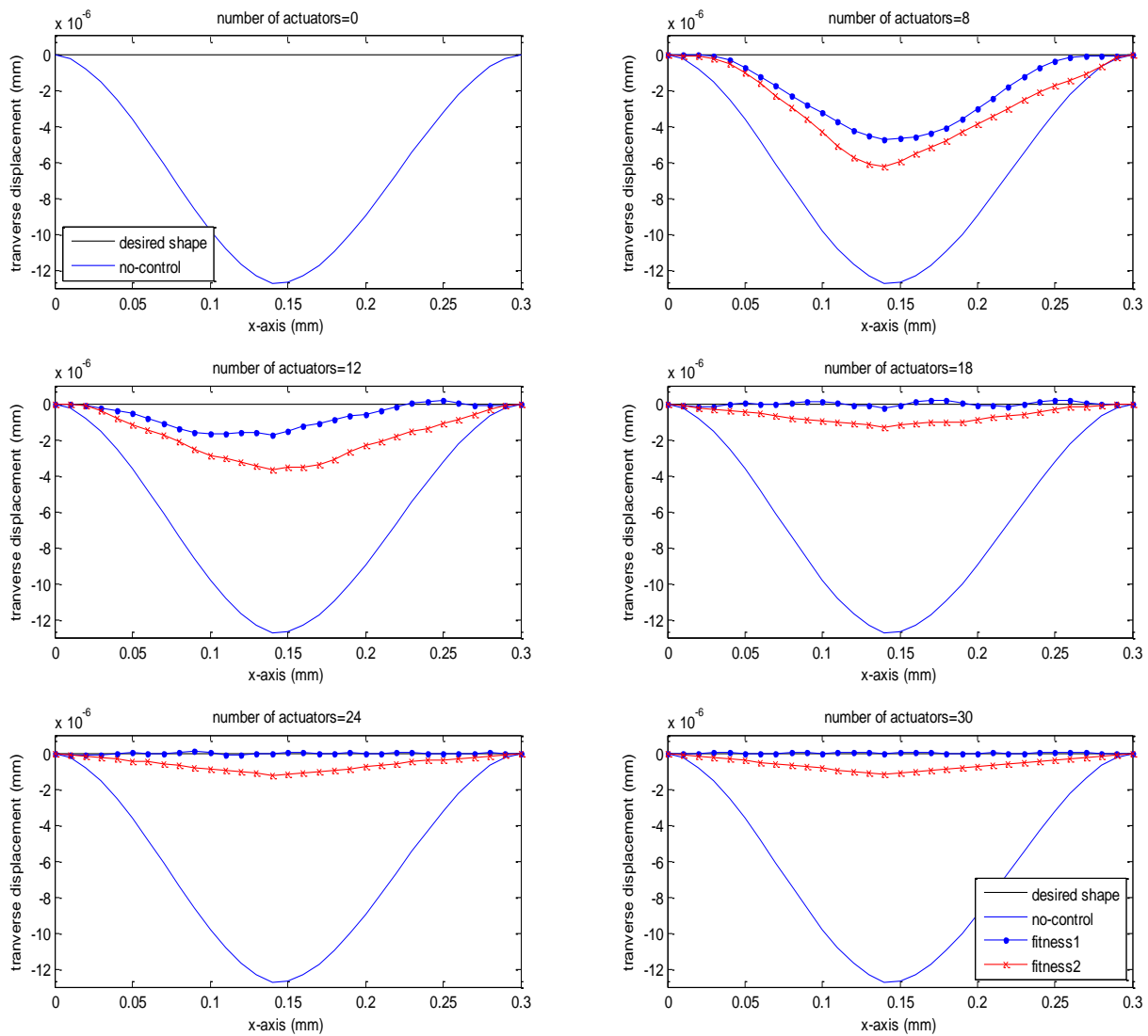
Figure 4. The centerline of the clamped–clamped smart beam under the action of various numbers of actuators for X^d(x) = 0 with the optimal values of actuation voltages.
