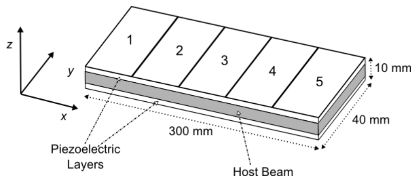
Figure 2. The smart beam structure.
