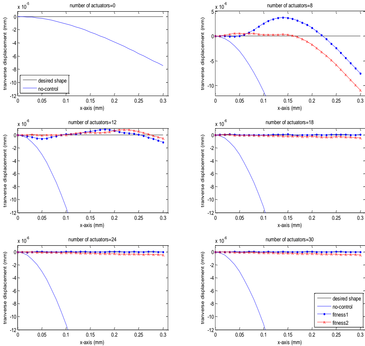
Figure 3. The centerline of the cantilever smart beam under the action of various numbers of actuators for X^d(x) = 0 with the optimal location of the actuators and the optimal values of actuation voltages.
