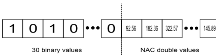
Figure 1. Chromosome encoding for the location and voltage problem.
