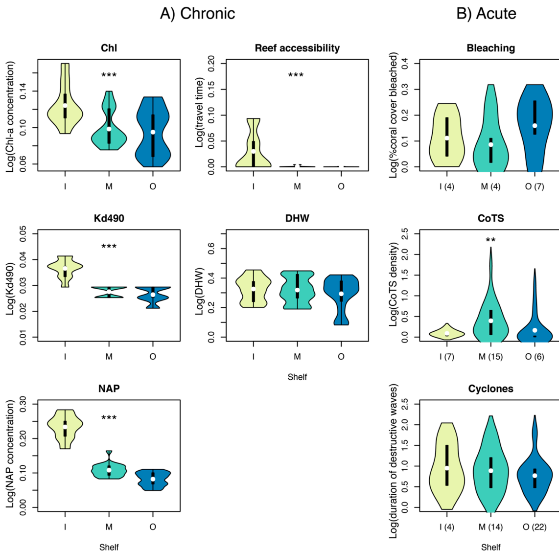
Figure 5. Distribution of chronic (A) and acute (B) stressors among inner (I), mid (M) and outer (O) shelf reefs. Violin plots represent data density, with plot width being proportional to the amount of data. Thick vertical lines represent the interquartile range, and the white dot the median. Asterisks show significant cross-shelf variation based on a Kruskal–Wallis test (***: P < 0.001 ; **: P < 0.01 ). For acute stressors, numbers in brackets represent the number of discrete disturbances. With Chl: long-term average of chlorophyll-a concentration; Kd490: light attenuation coefficient; NAP: non-algal particulates; DHW: Degree Heating Weeks; CoTS: outbreaks of the Crown-of-Thorns sea star ( Acanthaster cf. solaris ).
