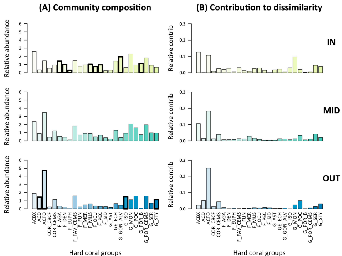
Figure 4. Composition of pre-disturbance hard coral communities (A) and relative contribution of each taxon to community dissimilarity (i.e., either disassembly or reassembly) following disturbance (B). Thick bar outlines in (A) show indicator taxa (Dufrene–Legendre index, P < 0.05 ) with, for inner-shelf reefs, F_AGA: encrusting, foliose and submassive Agariciidae; F_DEN: encrusting, foliose & massive Dendrophyllidae; F_EUPH: Euphyllidae; F_MUS: Mussidae; F_OCU: Oculinidae; F_PEC: Pectiniidae; G_GON_ALV: Goniopora and Alveopora ; G_MON: branching Porites ; and for outer-shelf reefs ACD: digitate Acropora ; ACTO: tabulate and corymbose Acropora ; G_ISO: encrusting and sub-massive Isopora ; G_STY: Stylophora . See Table 1 for other hard coral group codes and description.
