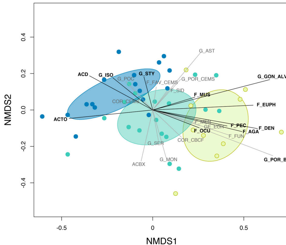
Figure 2. Non-metric multidimensional scaling of pre-disturbance communities at inner (yellow), mid (green) and outer (blue) shelf reefs (2D stress = 0.12). Dots show individual reefs, convex hulls delineate the different shelf assemblages (i.e., one standard deviation around the assemblage centroid) and segments show hard coral groups. Hard coral groups shown in black represent indicator taxa as per Figure 3. See Table 1 for hard coral group codes and description.
