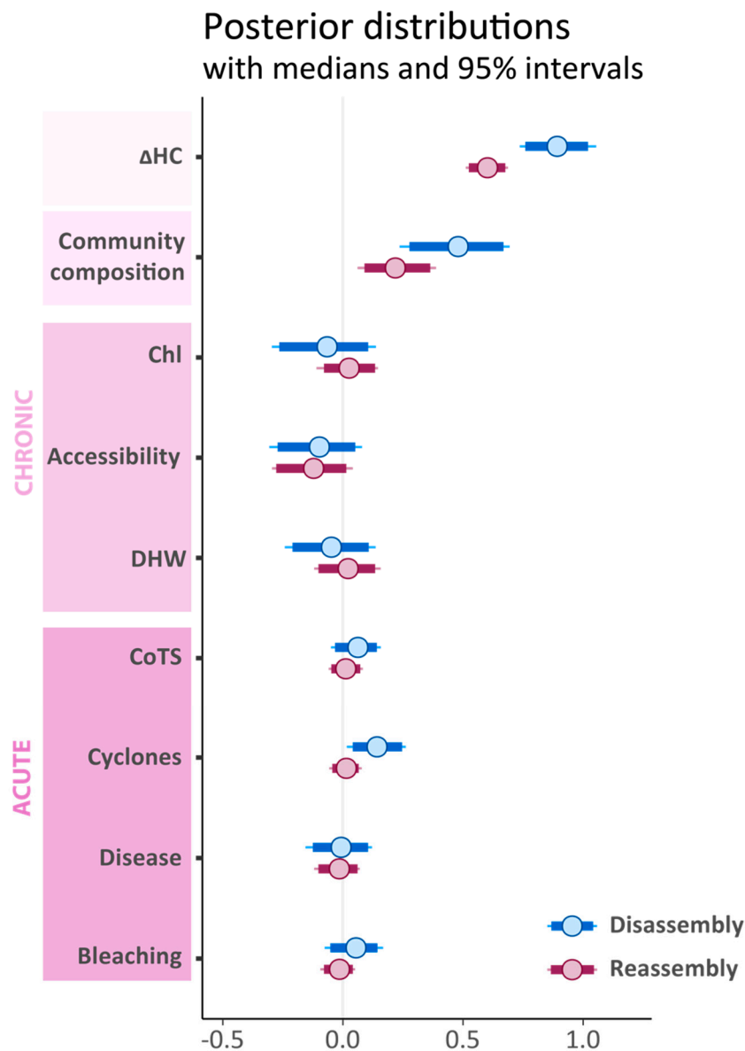
Figure 3. Posterior distributions of model coefficients (i.e., slopes) for fixed effects included in the Bayesian hierarchical models of community disassembly/reassembly following coral cover decline/recovery. Dots indicate the median, bars the 90% credible interval (CI) and whiskers the 95% CI. Where the 95% CI overlap zero, effects are considered non-significant. Community composition represents the first score of a non-metric multidimensional scaling of pre-disturbance communities (Supp. Figure 3). With \Delta HC : difference from maximum coral cover; Chl-a: long-term average of chlorophyll-a concentration; DHW: Degree Heating Weeks; CoTS: outbreaks of the Crown-of-Thorns sea star ( Acanthaster cf. solaris ).
