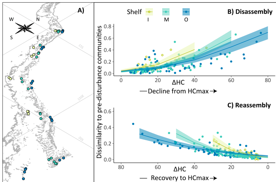
Figure 1. Coral community disassembly and reassembly across the continental shelf of Australia’s Great Barrier Reef. (A) Location of survey reefs, (B) hard coral community disassembly following coral cover decline (N = 144) and (C) coral community reassembly following coral cover recovery (N = 207) on inner-shelf (I), mid-shelf (M) and outer-shelf reefs (O). On (B,C), the y-axis represents the Bray–Curtis distance (dissimilarity) between disturbed and pre-disturbance community composition. ΔHC (%) represents the difference between the maximum coral cover observed at each reef and the coral cover measured at that reef in any given year. Envelopes show 95% credible intervals from the posterior distributions estimated from the Bayesian hierarchical model.
