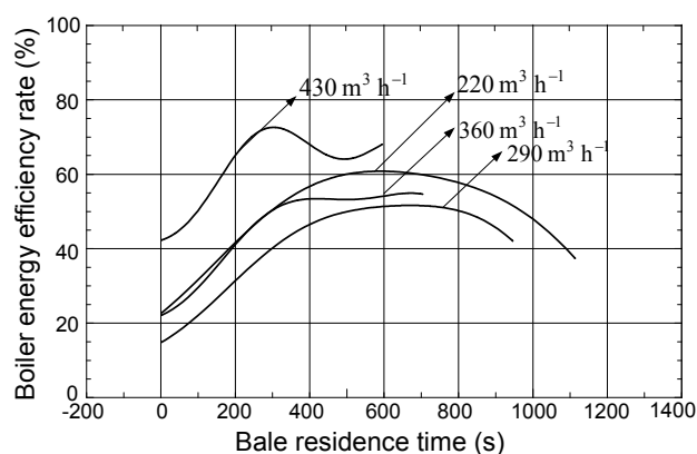
Figure 11. Correlation between boiler energy efficiency rate and bale residence time, model (7), recirculation 33%.
