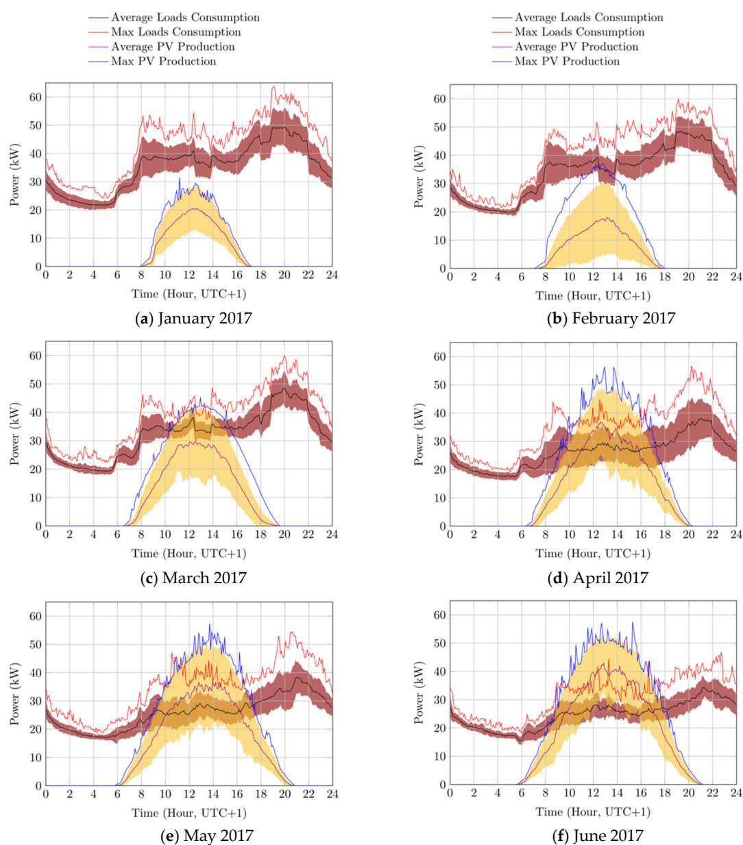
Figure 1. Monthly average and peak power data of photovoltaic (PV) production and user's loads recorded from January to June 2017, as depicted from sub-figure (a) to sub-figure (f), respectively. The yellow and red area represent the standard deviation of PV and loads data, respectively. UTC: Universal Time Coordinated.
