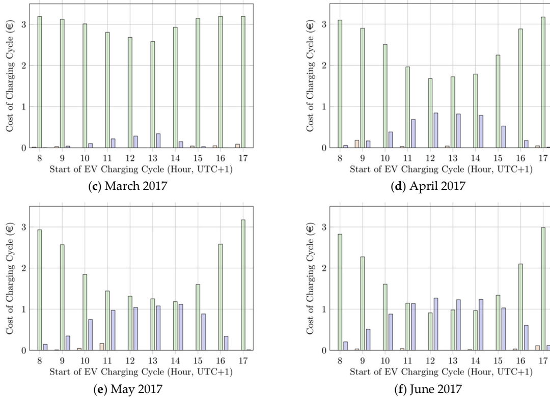
Figure 10. Electric vehicle (EV) charging cost components (€) from January to June 2017, as depicted from sub-figure (a) to sub-figure (f), respectively. The cost components are presented for each charging cycle, depending on the time of arrival of the EV at the charging station. UTC: Universal Time Coordinated.
