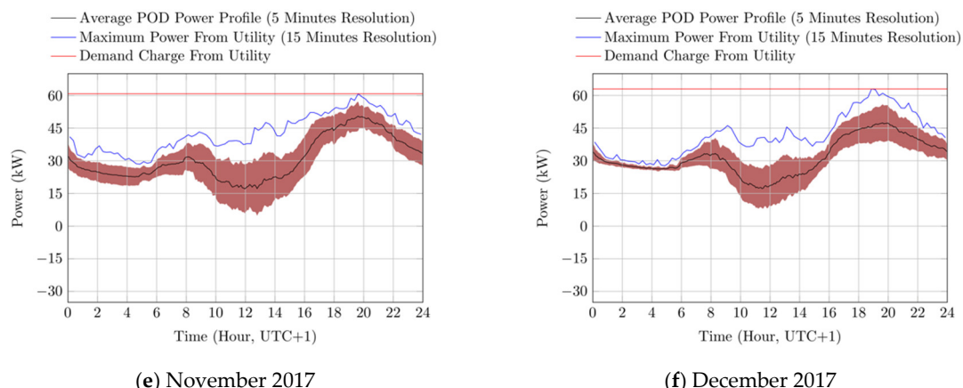
Figure 4. Monthly average and peak power data of the user’s point of delivery (POD), recorded from July to December 2017, as depicted from sub-figure (a) to sub-figure (f), respectively. Positive and negative values represent power flows from the grid and to the grid, respectively. Data are sampled every 10 s and the averages are recorded every 5 min. The red area represents the standard deviation of the measured POD power flows. UTC: Universal Time Coordinated.
