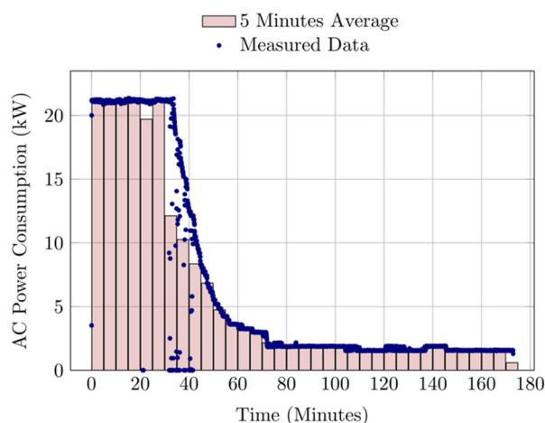
Figure 7. EV charging profile used as reference charging cycle in the simulations. EV: Electric Vehicle.
