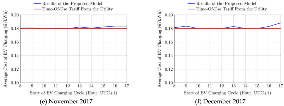
Figure 9. Monthly average cost of electric vehicle (EV) charging (€/kWh) from July to December 2017, as depicted from sub-figure (a) to sub-figure (f), respectively. The computed EV charging cost for each hour (blue line), is compared to the time-of-use (TOE) electricity tariff applied to the amount of energy purchased from the grid (red line). UTC: Universal Time Coordinated.
