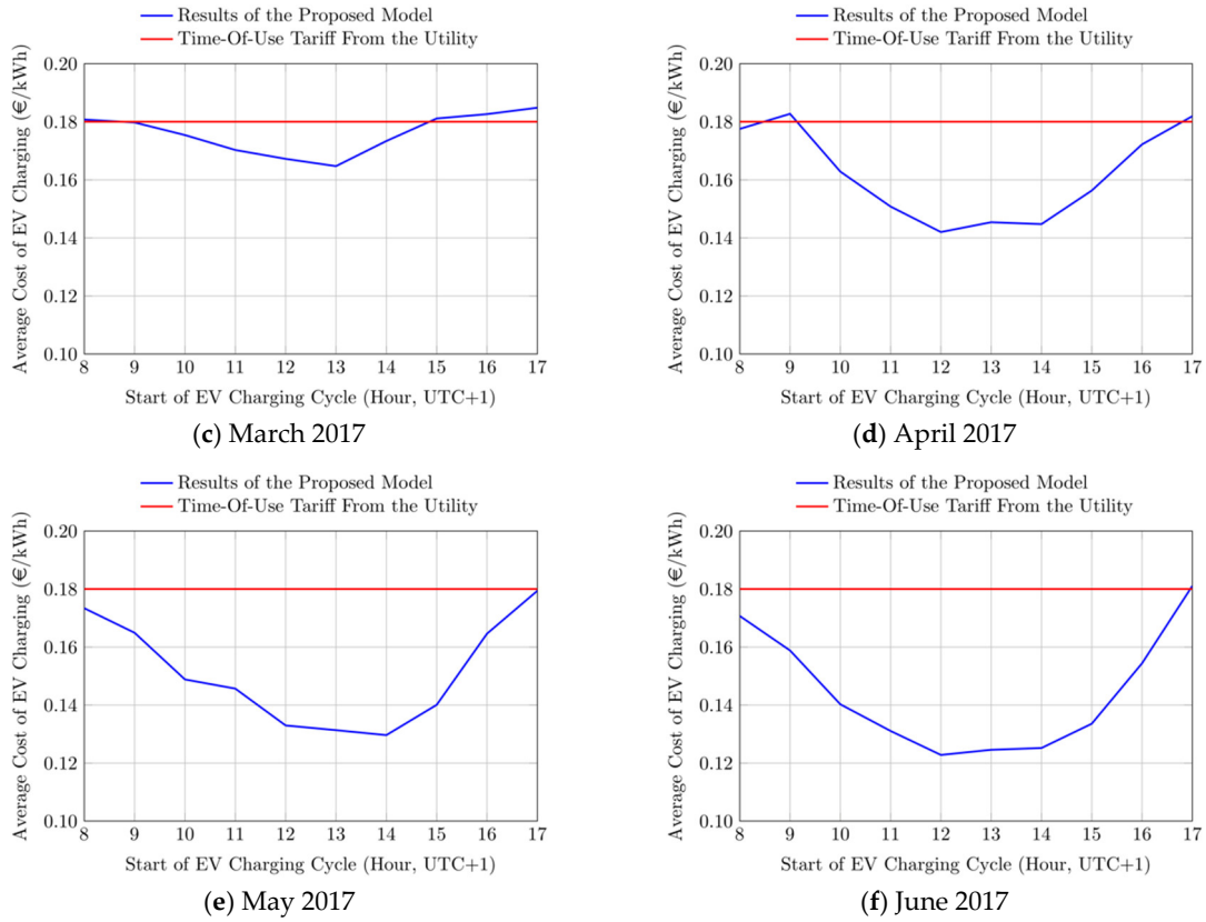
Figure 8. Monthly average cost of electric vehicle (EV) charging (€/kWh) from January to June 2017, as depicted from sub-figure (a) to sub-figure (f), respectively. The computed EV charging cost for each hour (blue line), is compared to the time-of-use (TOE) electricity tariff applied to the amount of energy purchased from the grid (red line). UTC: Universal Time Coordinated.
