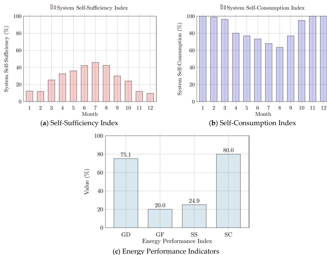
Figure 6. Energy key performance indicators (KPIs) of the system, based on data measured during 2017. In sub-figures (a) and (b) the self-sufficiency and the self-consumption of the system are reported for each month, respectively. In sub-figure (c), the grid-dependency (GD), grid-feed (GF), self-sufficiency (SS), and self-consumption (SC) indices are reported for the year 2017.
