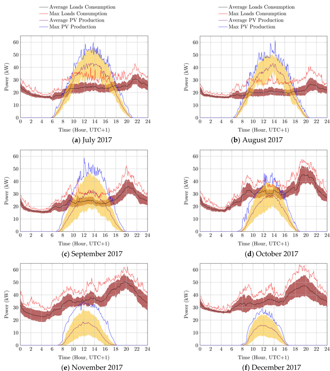
Figure 2. Monthly average and peak power data of photovoltaic (PV) production and user's loads recorded from July to December 2017, as depicted from sub-figure (a) to sub-figure (f), respectively. The yellow and red area represent the standard deviation of PV and loads data, respectively. UTC: Universal Time Coordinated.
