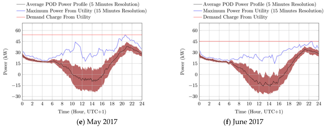
Figure 3. Monthly average and peak power data of the user’s point of delivery (POD), recorded from January to June 2017, as depicted from sub-figure (a) to sub-figure (f), respectively. Positive and negative values represent power flows from the grid and to the grid, respectively. Data are sampled every 10 s and the averages are recorded every 5 min. The red area represents the standard deviation of the measured POD power flows. UTC: Universal Time Coordinated.
