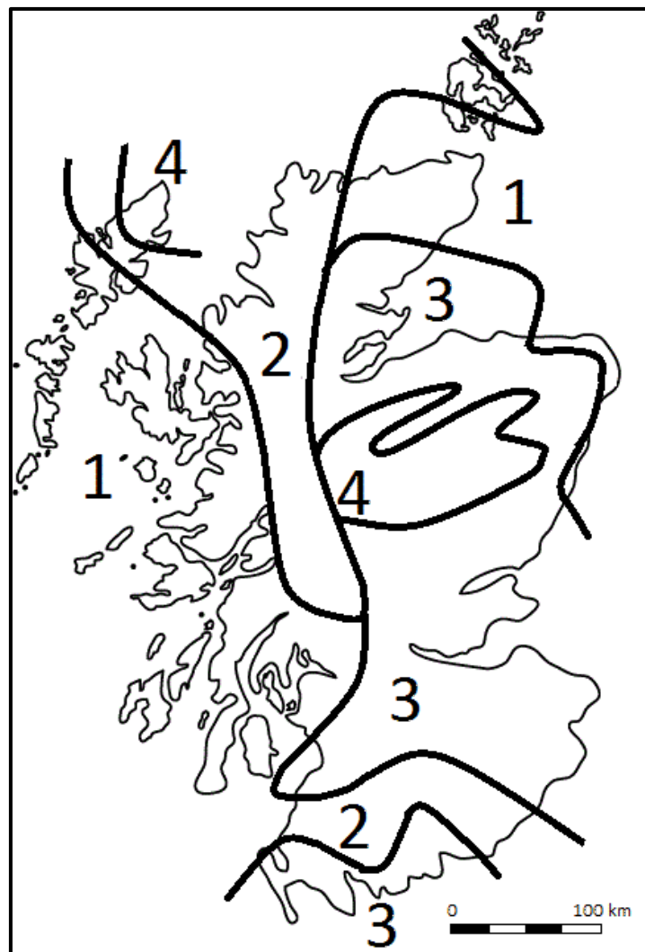
Figure 1. Sketch map of zones showing current and predicted suitability zones for Sitka spruce in Scotland by 2080. (1) remains largely suitable; (2) partially suitable becoming more suitable; (3) partially suitable becoming largely unsuitable; (4) remains largely unsuitable. Based on a simplified version of data presented in Ray [2].
