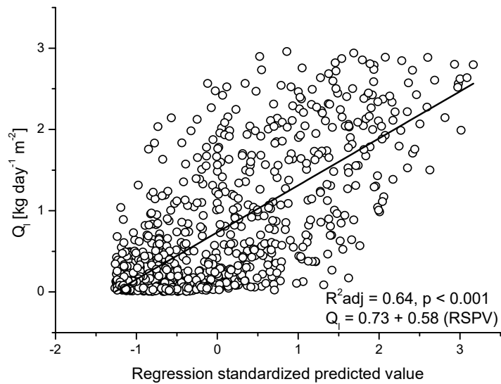
Figure 7. Regression model describing the combined effect of vapor pressure deficit (VPD) [kPa] and net radiation [ \text{kWm}^{-2} ] on Q_l . Mean hourly values of VPD and net radiation corresponding to the days' sap flow was monitored during the wet period (November to March) were used. RSPV stands for regression standardized predicted value.
