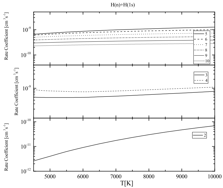
Figure 2. Plot of the rate coefficients for collisional ionisation H^*(n) + H(1s) (i.e., for chemi-ionization processes (1)) as a function of n and T .
