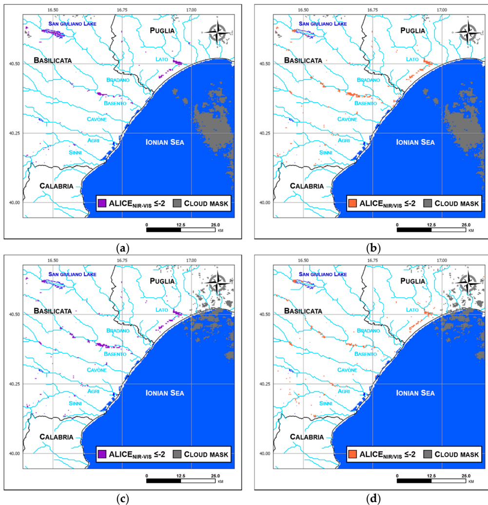
Figure 5. Anomalous pixels detected by Visible Infrared Imaging Radiometer Suite (VIIRS)-based RST-FLOOD using: (a) ALICE_{NIR-VIS} , (b) ALICE_{NIR/VIS} on 4 December 2013 at 12:10 GMT and (c) ALICE_{NIR-VIS} , (d) ALICE_{NIR/VIS} on 5 December 2013 at 11:50 GMT.
