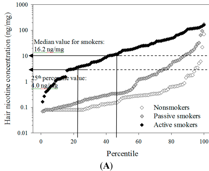
Figure 2. Distributions of hair nicotine and salivary cotinine concentrations by self-reported smoking status and 25th and 50th percentile values obtained from self-reported active smokers. Three different shades (black, gray, and white) represent for active smokers, passive smokers and nonsmokers, separately.) (A) Hair nicotine; (B) Salivary cotinine.
