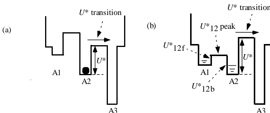
Figure 3. Potential of the force exerted on the myosin head in the MA 3 complex. The shape varies depending upon the tension T . (a) The case of T < T_{dev} , where the force-velocity relation is Hill-type. The black circle indicates that the myosin head exists solely in well A2; (b) The case of T_{dev} < T < T_{obs} , where the existence probability of the myosin head is distributed in wells A1 and A2, causing deviation of the force-velocity relation from Hill-type.
