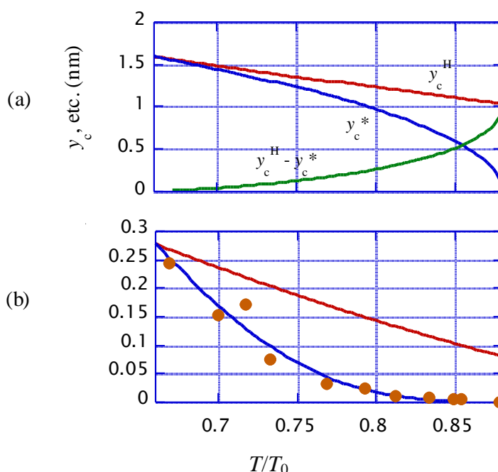
Figure 19. Explanation of the deviation of the force-velocity relation from Hill-type. (a) y_c^H, y_c^*, y_c^H - y_c^* as functions of T/T_0 , calculated by Equations 51 and 52; (b) Brown circles: Experimental data of the sliding velocity per half sarcomere cited from Fig. 3A of the paper by Edman [12]. Red curve: v^H , the Hill-type velocity calculated in [2]. Blue curve: v^* , the velocity in the presence of the U^*_{12} transition calculated by Equations 53 and 54.
