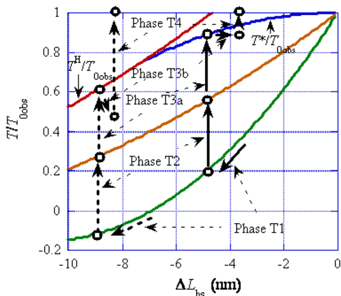
Figure 13. Phases in the isometric tension transient on the T/T_{0obs} vs. \Delta L_{hs} relation. The thick black solid and dashed arrows, respectively, indicate Phases in the cases of \Delta y_{cT1} < y_{cdev} and \Delta y_{cT1} > y_{cdev} . Actually the thick solid and dashed arrows are on the same vertical lines, respectively, except for the case of Phase T1.
