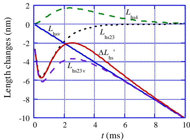
Figure 17. Characteristics of L_{hs4} , L_{hsv} , L_{hs23} , L_{hs23v} and \Delta L_{hs}' are illustrated in the case of \Delta T/T_{0obs} = (T_{0obs} - T)/T_{0obs} = 0.87 , by using the equations and parameter values given in text.
