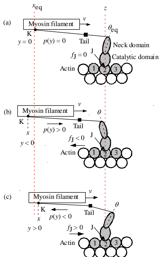
Figure 4. Definition of y , the shortening of the crossbridge: y = x - x_{eq} (after Figure 4 of [2]). The binding positions J are set on the dotted red line z . (a) The myosin head is at its equilibrium angle, \theta_{eq} . x = x_{eq} and y = 0 ; (b) The myosin head is pulling the myosin filament forward. The crossbridge is elongated and y < 0 ; (c) The myosin head is pushing the myosin filament backward. The crossbridge is shortened and y > 0 .
