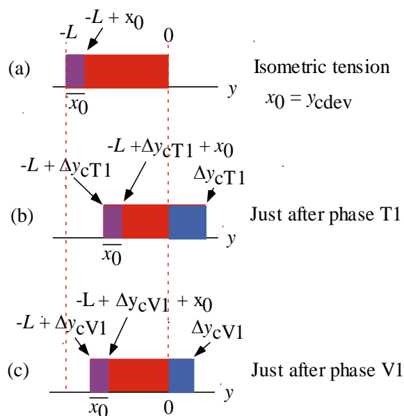
Figure 10. The \rho distributions before and after instantaneous changes in the isometric tension transient and in the isotonic velocity transient. (a) The isometric tetanus state; (b) Just after Phase T1 in the isometric tension transient; (c) Just after Phase V1 in the isotonic velocity transient for the same length change as (b).
