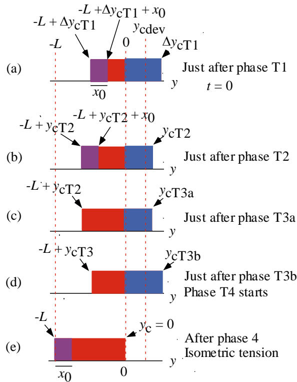
Figure 12. Changes of the \rho distribution during the isometric tension transient in the case of \Delta y_{cT1} > y_{cdev} .
