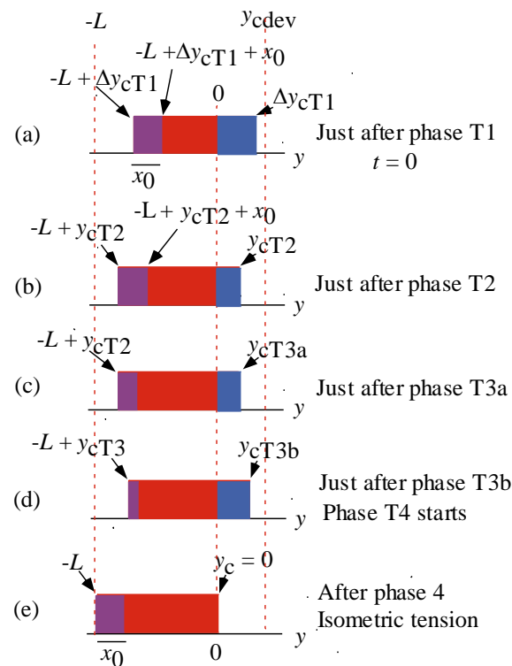
Figure 11. Changes of the \rho distribution during the isometric tension transient in the case of \Delta y_{cT1} < y_{cdev} . Magnitude of y_{cdev} is exaggerated for illustration.
