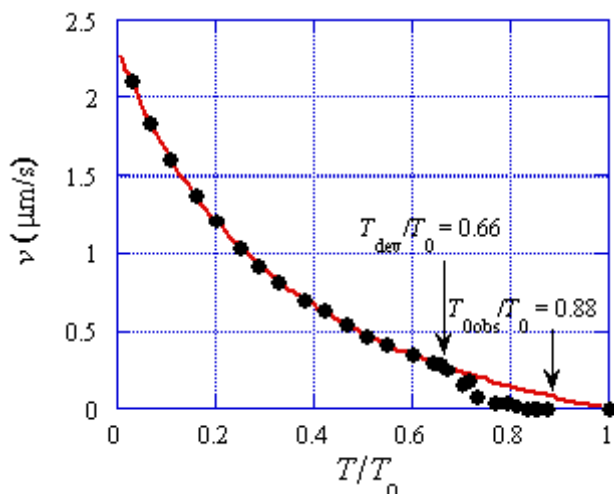
Figure 1. Force-velocity relation and definition of T_{dev} and T_{0obs} . The red curve is the calculation result reported in [2], which coincides with the hyperbolic force-velocity relation proposed by Hill [10]. Circles are the experimental results cited from Figure 6A of the paper by Edman [12].
