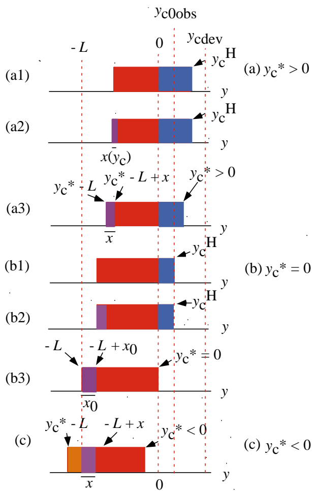
Figure 7. Compensation of the effect of the U_{12}^* transition by shift of y_c^H to y_c^* . Magnitudes of y_{c0obs} and y_{cdev} are exaggerated for illustration. (a) y_{c0obs} < y_c^H < y_{cdev} and y_c^* > 0 ; (b) y_c^* = 0 ; (c) y_c^* < 0 .
