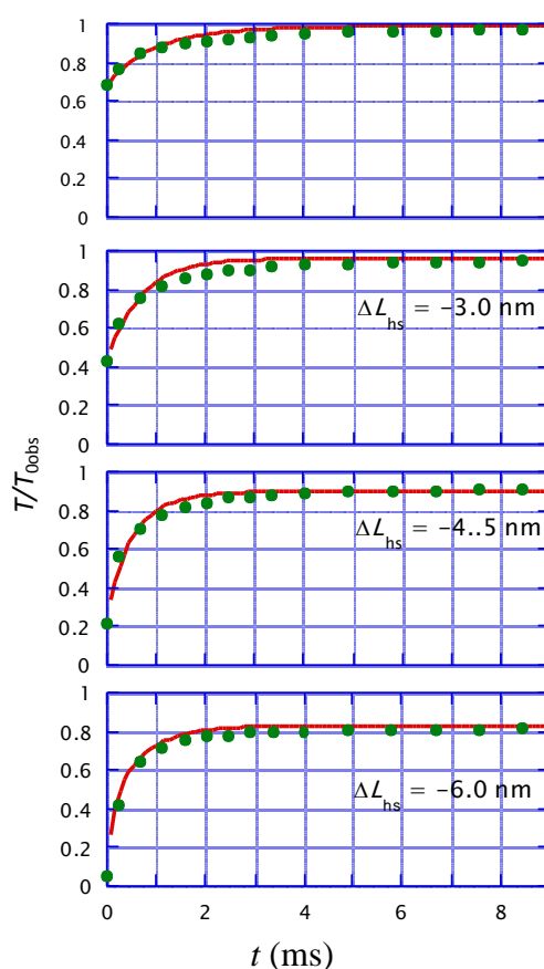
Figure 14. T/T_{0obs} as functions of time t for various length change steps \Delta L_{hs} in the isometric tension transient. The origin of t is set as the moment that Phase T1 finishes. Green circles: Experimental data cited from Figure 23 of Ford et al. [16]. Red lines: Values of T_{123a}/T_{0obs} calculated by using Equations 34, 35, 36 and the parameter values in Equation 38.
