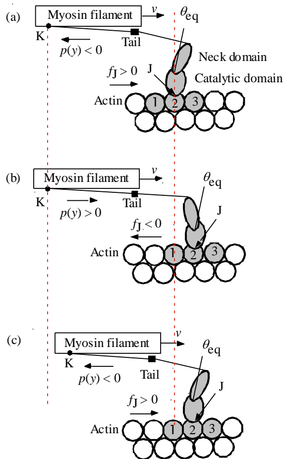
Figure 2. MA 3 complex (shadowed) and its step motion along the actin filament (after Figure 6 of [2]). A myosin head is expressed as neck domain plus catalytic domain and the actin molecules in MA 3 as 1, 2 and 3. (a) Just before the myosin head moves to the right; (b) Just after the head (and the complex MA 3 ) moves to the new position; (c) The head is ready for next movement to the right. (Note that the actin molecule bound to a myosin molecule is called 2.)
