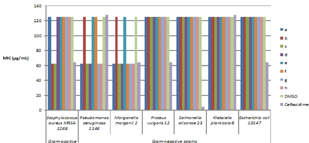
Figure 1. Minimum inhibitory concentration (MIC) of dibenz[ b,e ]oxepins.
