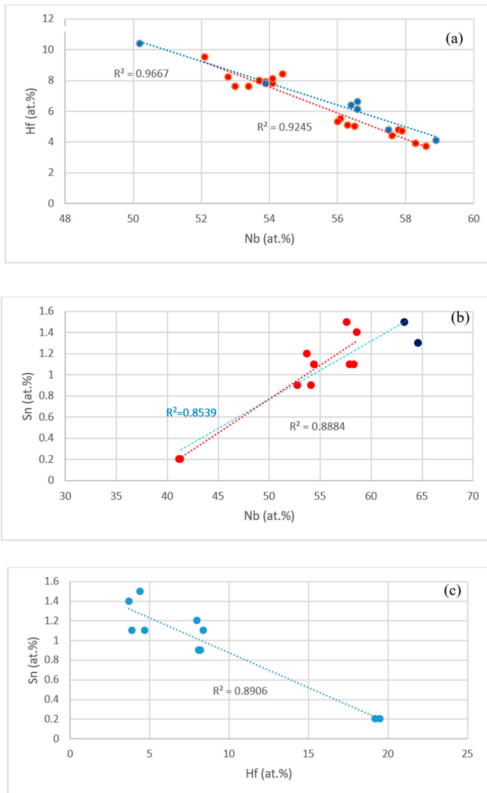
Figure 10. (a) Hf (ordinate) versus Nb (abscissa) in Nb_5Si_3 and Hf rich Nb_5Si_3 for the alloys EZ1, EZ3, EZ4 (red data points) and Nb-18Si-5Cr-5Hf (YG1 [17]) and Nb-18Si-5Al-5Hf (YG2 [17]) (blue data points), (b) Sn (ordinate) versus Nb (abscissa) in Nb_5Si_3 in the Al containing alloys EZ4 and EZ7. Data for alloy EZ4 is shown in red. All data R^2 = 0.8539 , data for the alloy EZ4 R^2 = 0.8884 , (c) Sn (ordinate) versus Hf (abscissa) in Nb_5Si_3 in the Al containing alloy EZ4.
