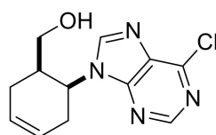
((1R*,6S*)-6-(6-Chloro-9H-purin-9-yl)cyclohex-3-en-1-yl)methanol, (±)-43.
