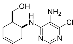
((1R*,6S*)-6-((5-Amino-6-chloropyrimidin-4-yl)amino)cyclohex-3-en-1-yl)methanol, (±)-42.
