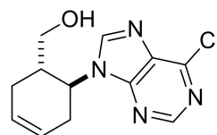
((1S*,6S*)-6-(6-Chloro-9H-purin-9-yl)cyclohex-3-en-1-yl)methanol, (±)-47.
