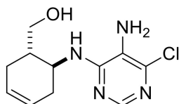
((1S*,6S*)-6-((5-Amino-6-chloropyrimidin-4-yl)amino)cyclohex-3-en-1-yl)methanol, (±)-46.
