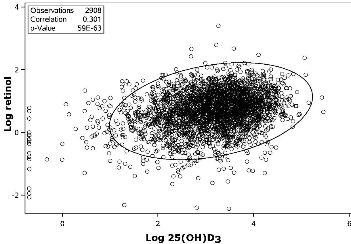
Supplementary Figure 1: Scatterplot with 95% confidence ellipse for log 25(OH)D 3 vs log retinol
