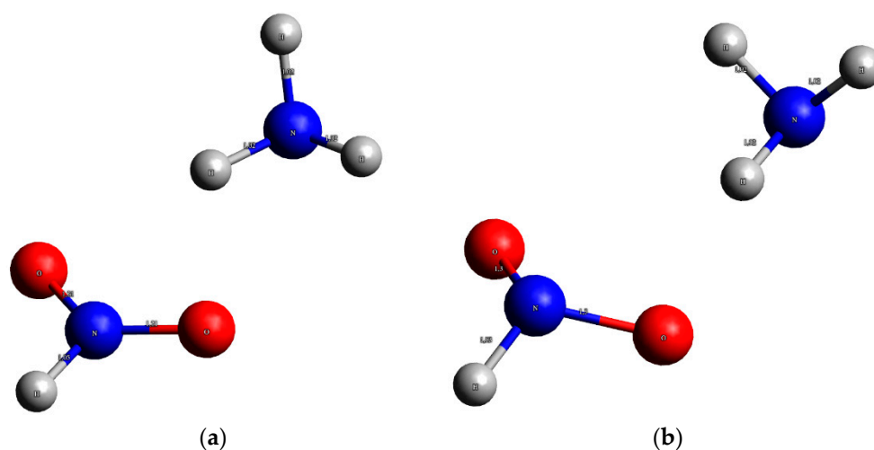
Figure 1. \text{HNO}_2 + \text{NH}_3 geometry in (a) singlet (b) triplet state.
