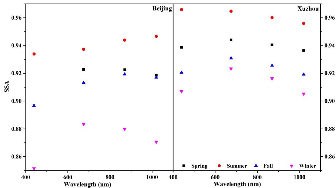
Figure S2. Seasonal averaged SSA with AOD 440 nm > 0.4 on HPDs in Beijing and Xuzhou.
