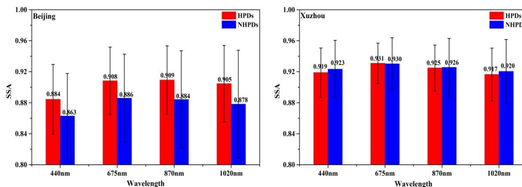
Figure S1. Averaged SSA with AOD 440 nm > 0.4 on HPDs and NHPDs in Beijing and Xuzhou.
