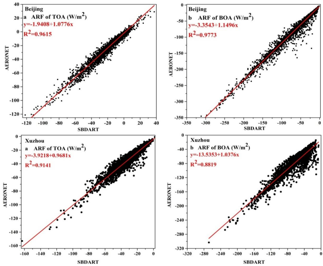
Figure S3. Comparison between SBDART-simulated and AERONET-retrieved direct aerosol radiative forcing.
