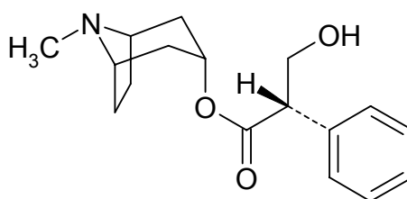
Fig. 1. Example for the chemical structure of a compound [Arial 12, left alignment]
