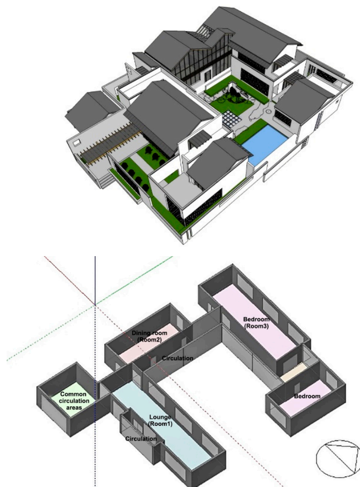
Figure 6. The simulation model of the courtyard building.
