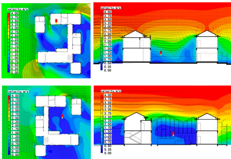
Figure 8. The sectional plan of the wind speed contour of the courtyard in winter under the initial design (top) and improved design (below).
