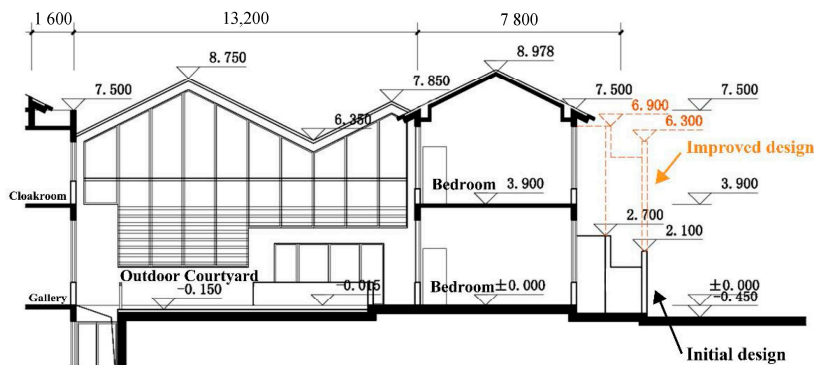
Figure 4. Illustration of the initial design and the improved design.
