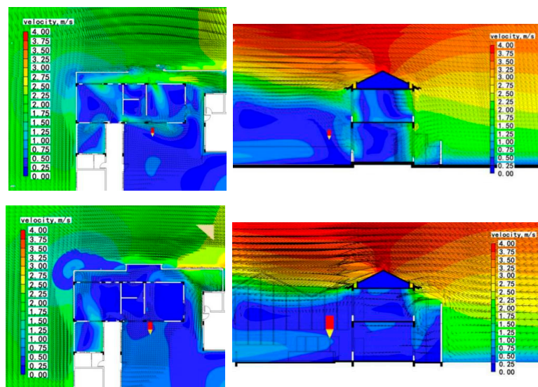
Figure 10. The sectional plan of the wind speed contour in winter under the initial design ( top ) and improved design ( below ).
