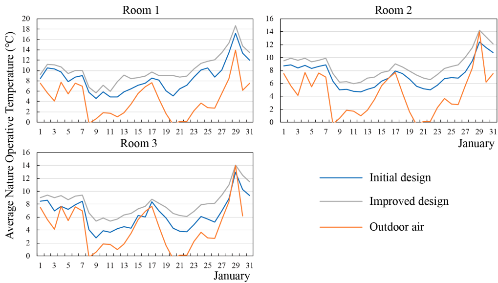
Figure 12. The average nature temperature results for three rooms in winter for initial design, improved design, and outdoor air.
