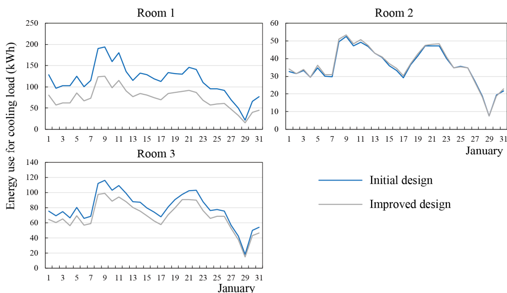
Figure 14. The energy use for thermal loads in rooms 1, 2, and 3 in winter under the initial design and improved design.
