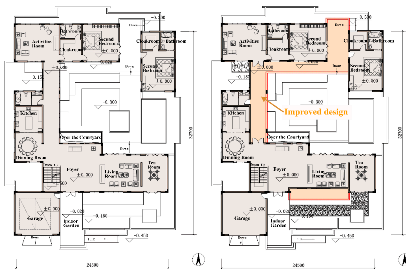
Figure 5. The ecological buffer spaces: Initial design (left), improved design (right).
