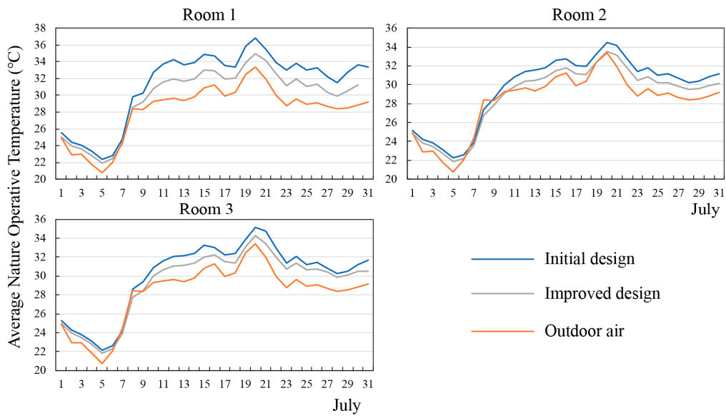
Figure 11. The average nature temperature results for three rooms in summer for initial design, improved design, and outdoor air.
