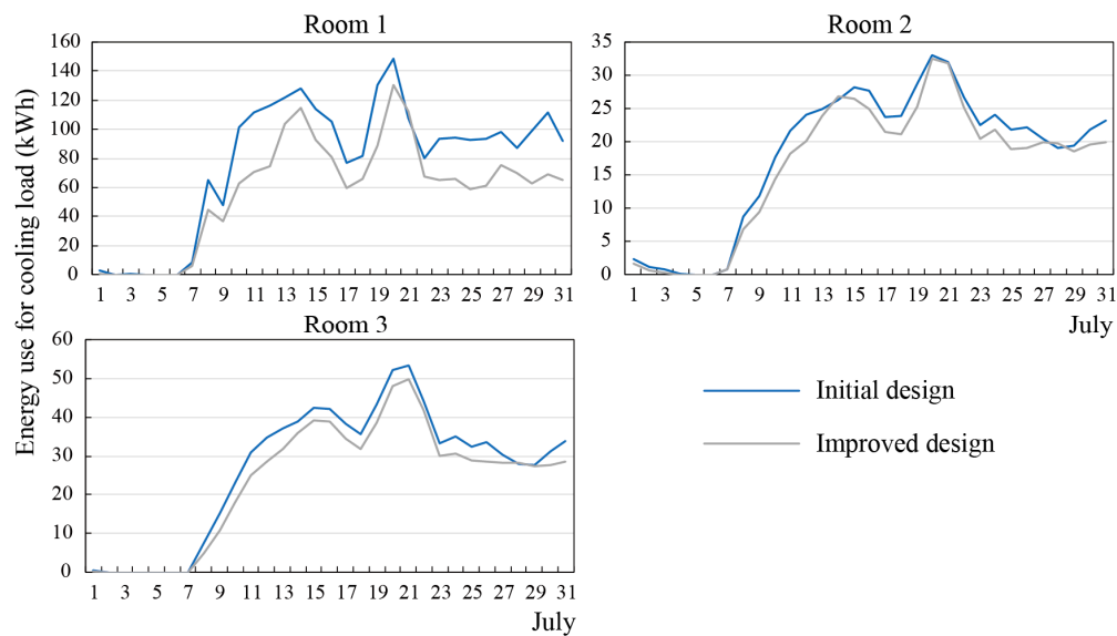
Figure 13. The energy use for thermal loads in rooms 1, 2, and 3 in summer under the initial design and improved design.
