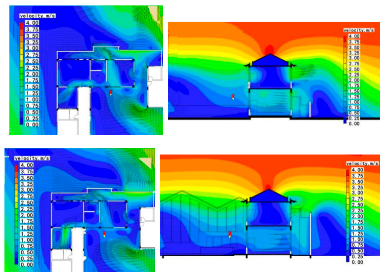
Figure 9. The sectional plan of the wind speed contour in summer under the initial design ( top ) and improved design ( below ).
