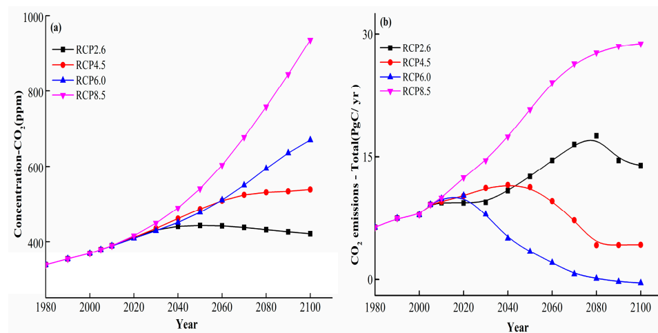
Figure 2. Global carbon dioxide ( CO_2 ) concentration and emission for each representative concentration pathway (RCP) scenario (2.6, 4.5, 6.0, and 8.5) from the years 1980 to 2100. (a) Description of changing CO_2 concentrations; (b) description of changing CO_2 emissions.
