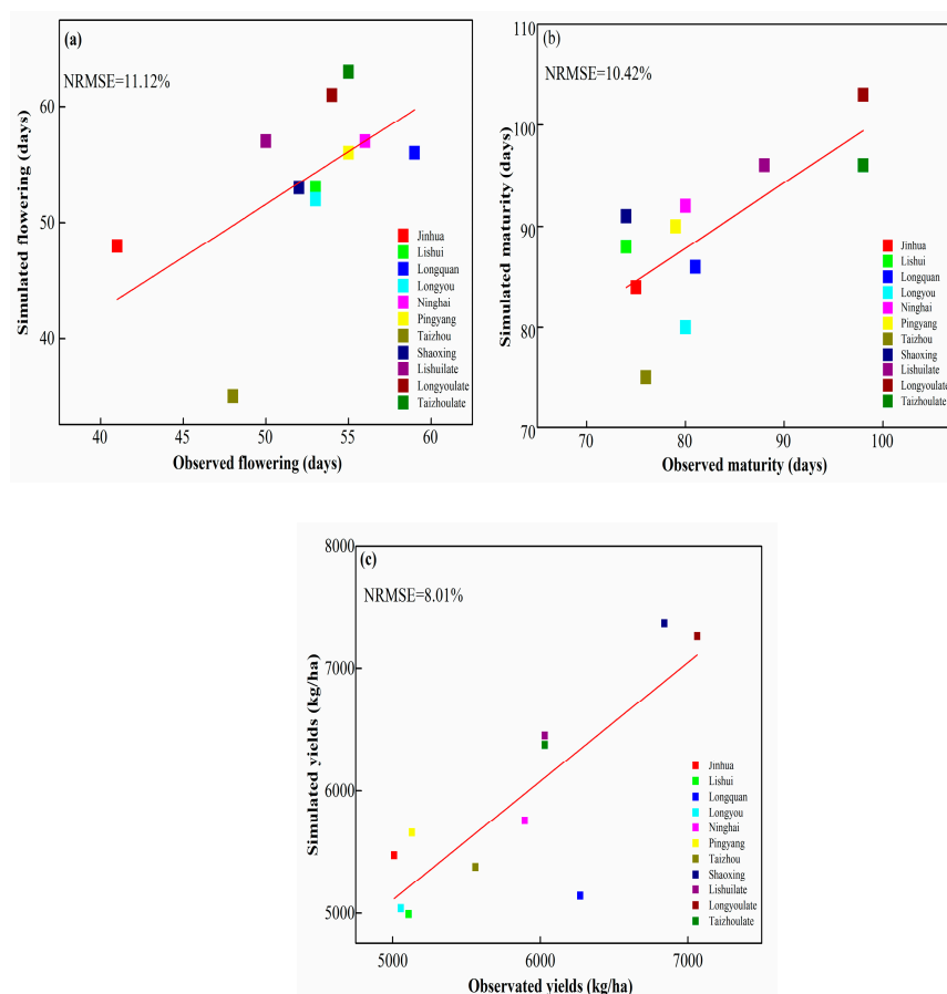
Figure 4. Simulated and observed flowering period, maturation period, and yields at all sites. (a) Calibration results for the flowering period; (b) calibration results for the maturation period; and (c) calibration results for the rice yields.
