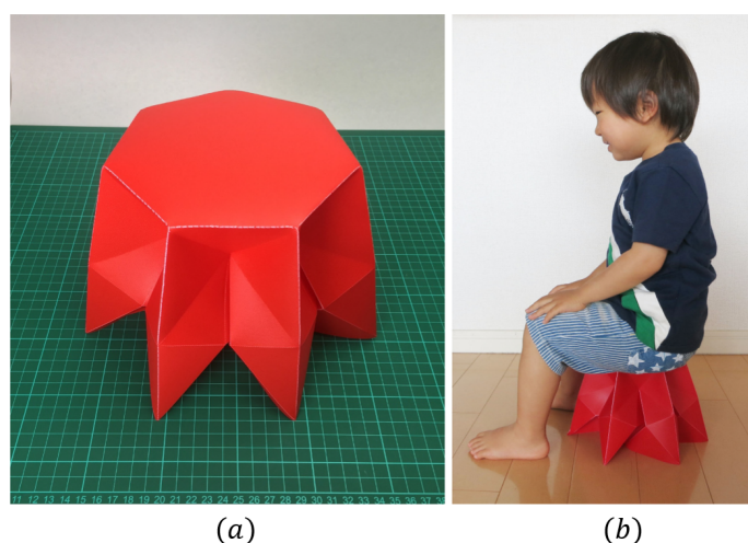
Figure 11. Load bearing experiment on stool shape-like origami with tucks inside. (a) An origami stool using polypropylene with 0.75 mm thickness; (b) A two-year-old boy of 13 kg could sit on the stool.
