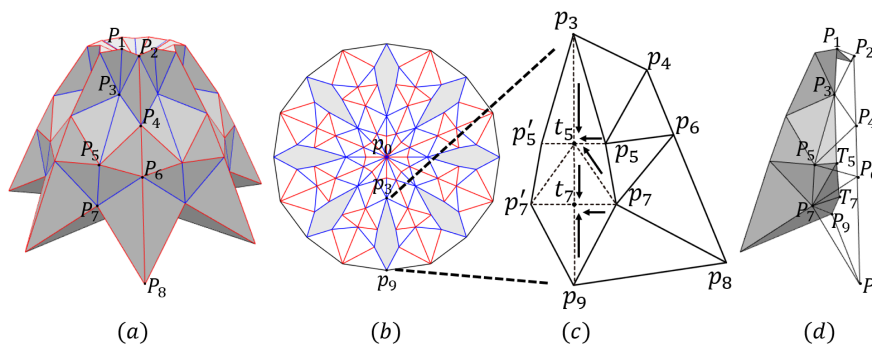
Figure 8. Calculating 3D flaps folded from polygonal blank spaces: (a) edited 3D origami; (b) the crease pattern whose blank spaces are polygons; (c) handling the blank space; (d) the calculated tuck inside the shape.
